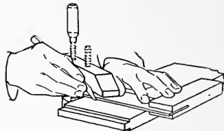
FIG. 339. CUTTING ACROSS THE GRAIN.
